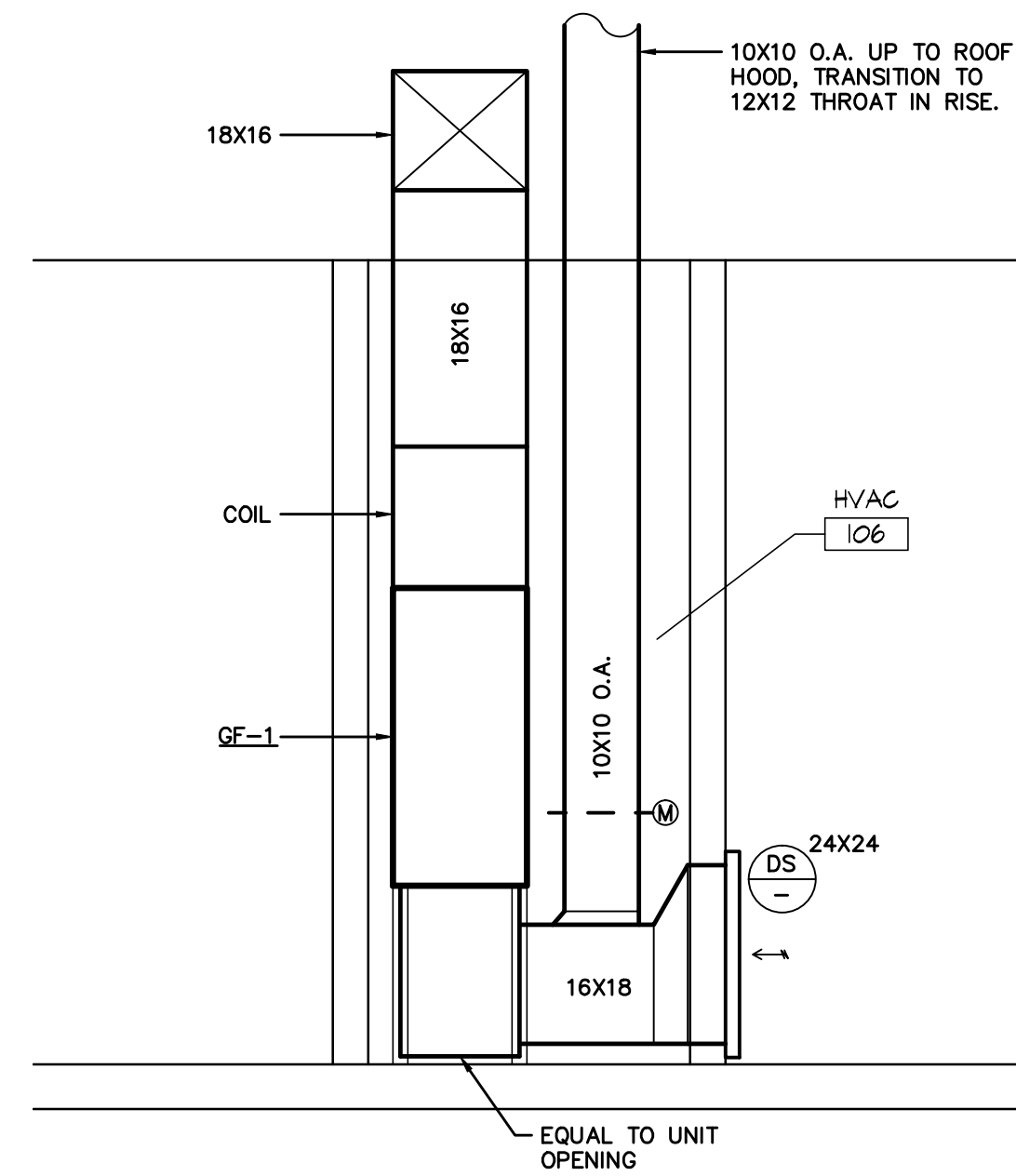
2 SECTION AT GAS FURNACE M-1.1 SCALE: 1/2" = 1'-0"
