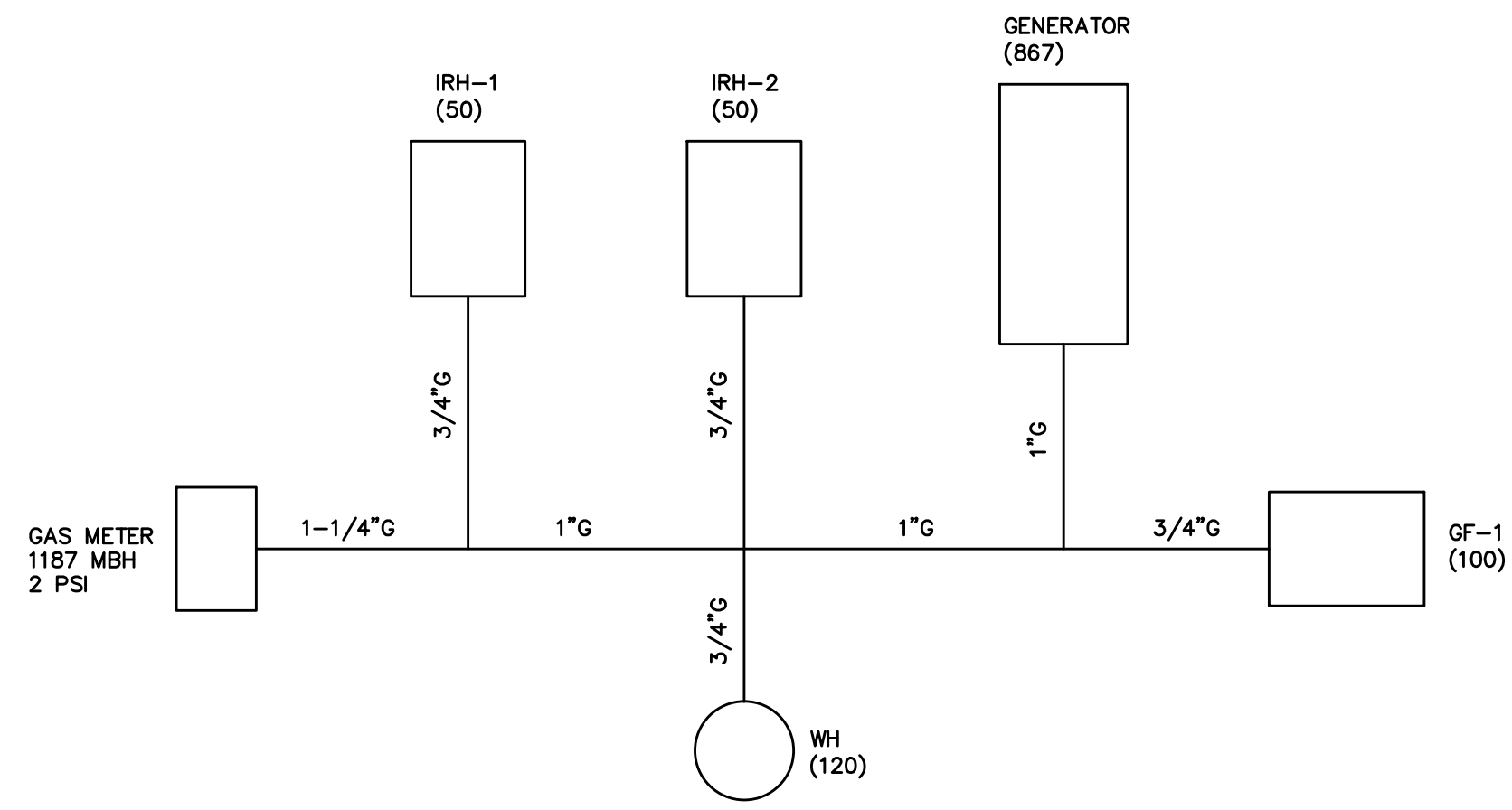
3 GAS PIPING SCHEMATIC M-1.1 NTS
