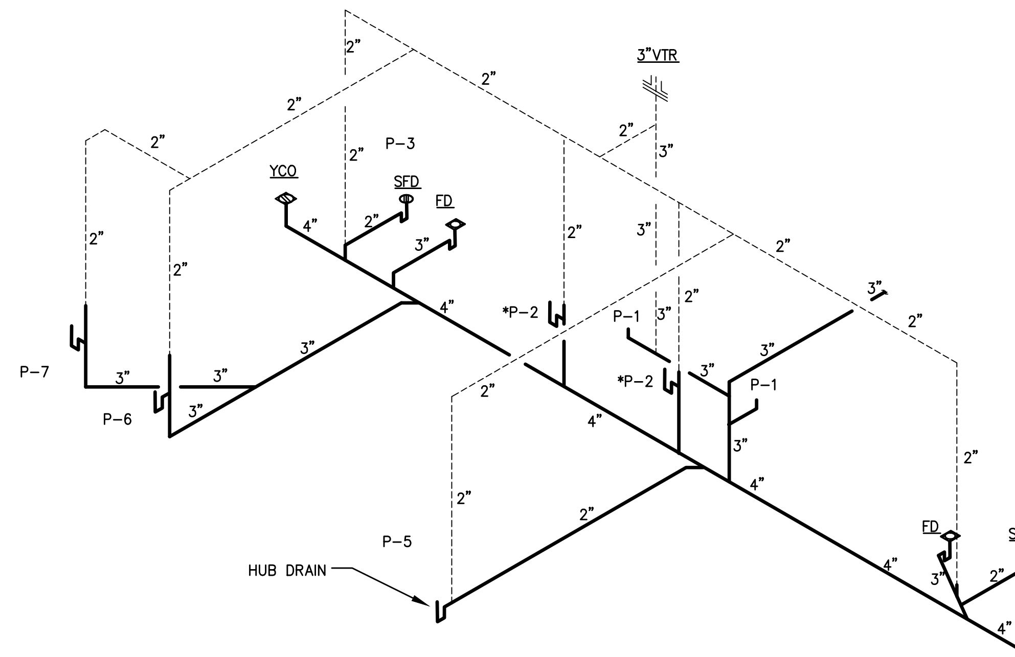
2 WASTE PIPING SCHEMATIC P-1.1 NTS
