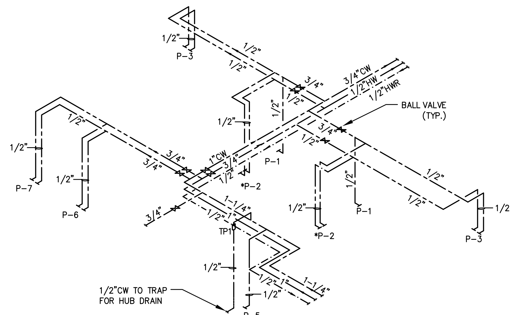
3 WATER PIPING SCHEMATIC P-1.1 NTS
